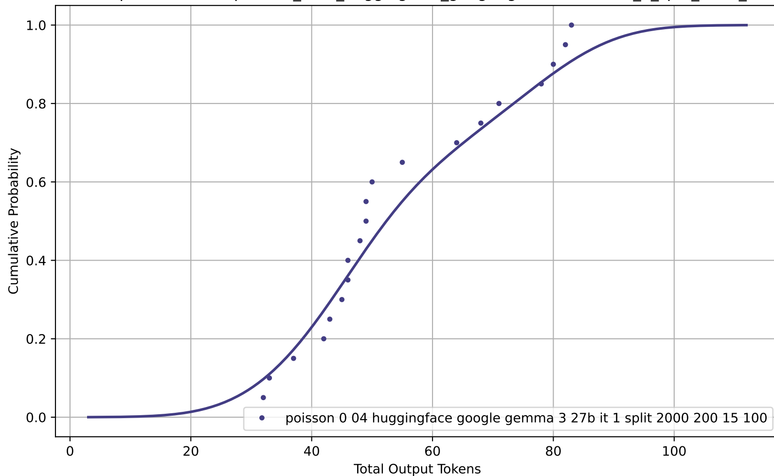
CDF of Total Output Tokens for poisson_0-04_huggingface_google-gemma-3-27b-it_1_split_2000_200_15_100
