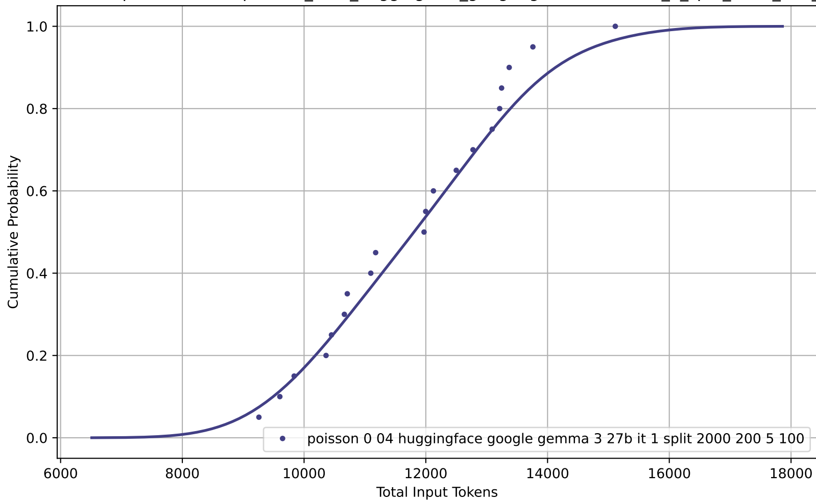
CDF of Total Input Tokens for poisson_0-04_huggingface_google-gemma-3-27b-it_1_split_2000_200_5_100
