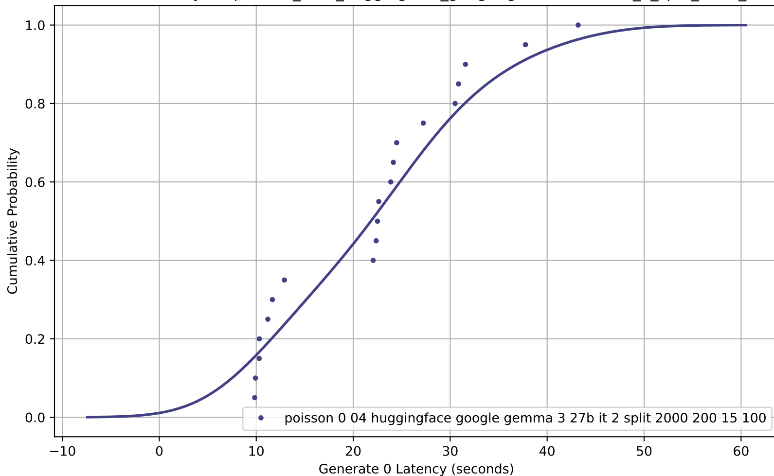
CDF of Generate 0 Latency for poisson_0-04_huggingface_google-gemma-3-27b-it_2_split_2000_200_15_100
