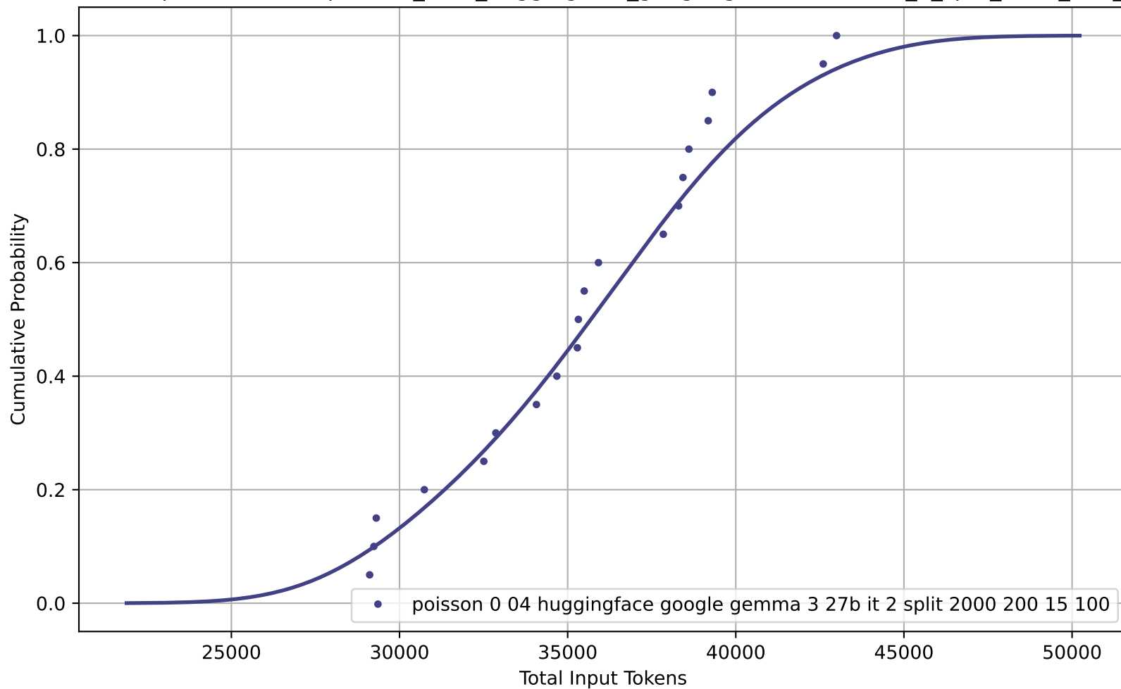
CDF of Total Input Tokens for poisson_0-04_huggingface_google-gemma-3-27b-it_2_split_2000_200_15_100
