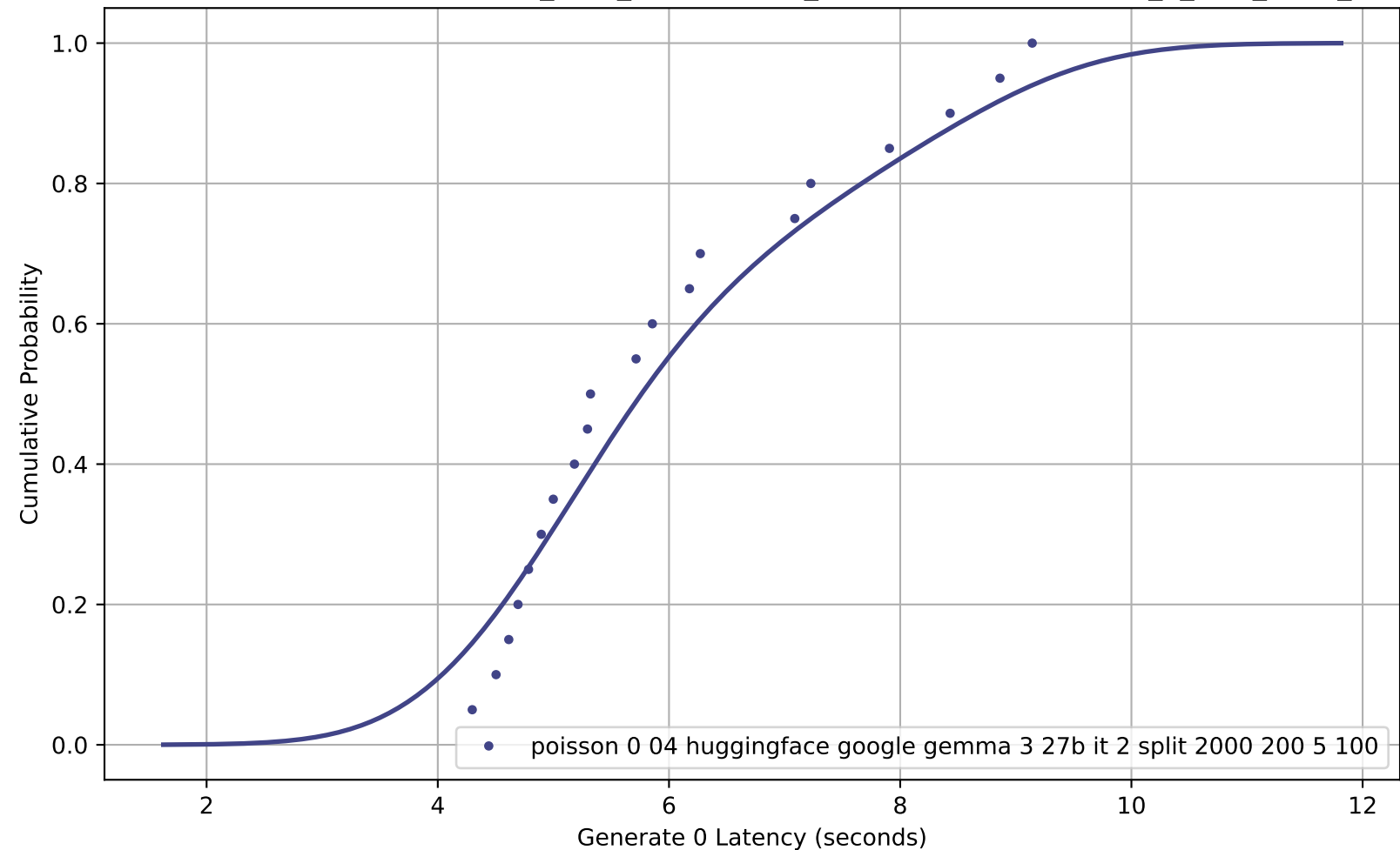
CDF of Generate 0 Latency for poisson_0-04_huggingface_google-gemma-3-27b-it_2_split_2000_200_5_100
