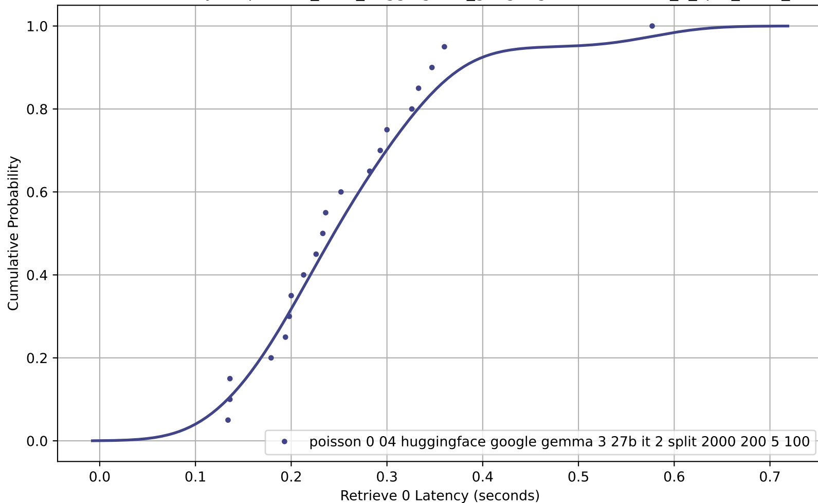
CDF of Retrieve 0 Latency for poisson_0-04_huggingface_google-gemma-3-27b-it_2_split_2000_200_5_100
