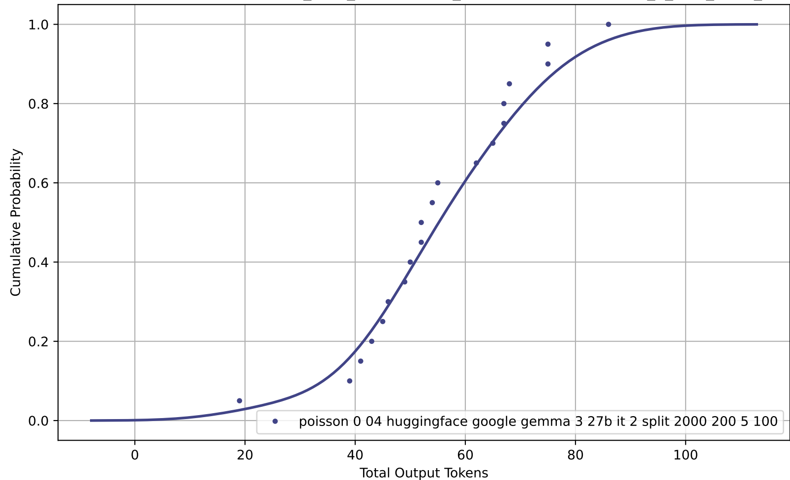
CDF of Total Output Tokens for poisson_0-04_huggingface_google-gemma-3-27b-it_2_split_2000_200_5_100
