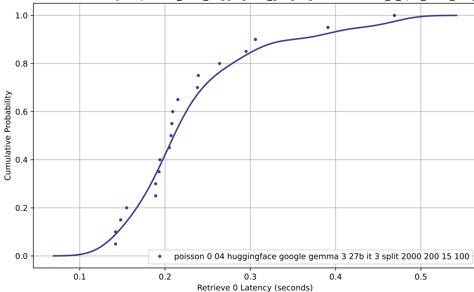
CDF of Retrieve 0 Latency for poisson_0-04_huggingface_google-gemma-3-27b-it_3_split_2000_200_15_100
