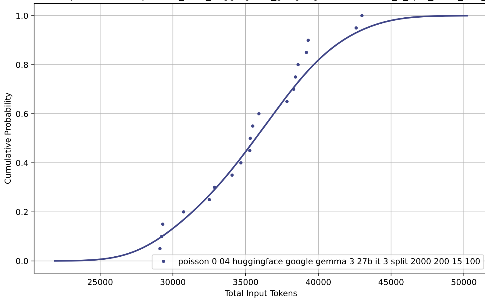
CDF of Total Input Tokens for poisson_0-04_huggingface_google-gemma-3-27b-it_3_split_2000_200_15_100
