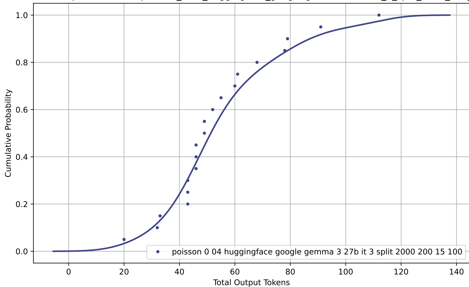
CDF of Total Output Tokens for poisson_0-04_huggingface_google-gemma-3-27b-it_3_split_2000_200_15_100
