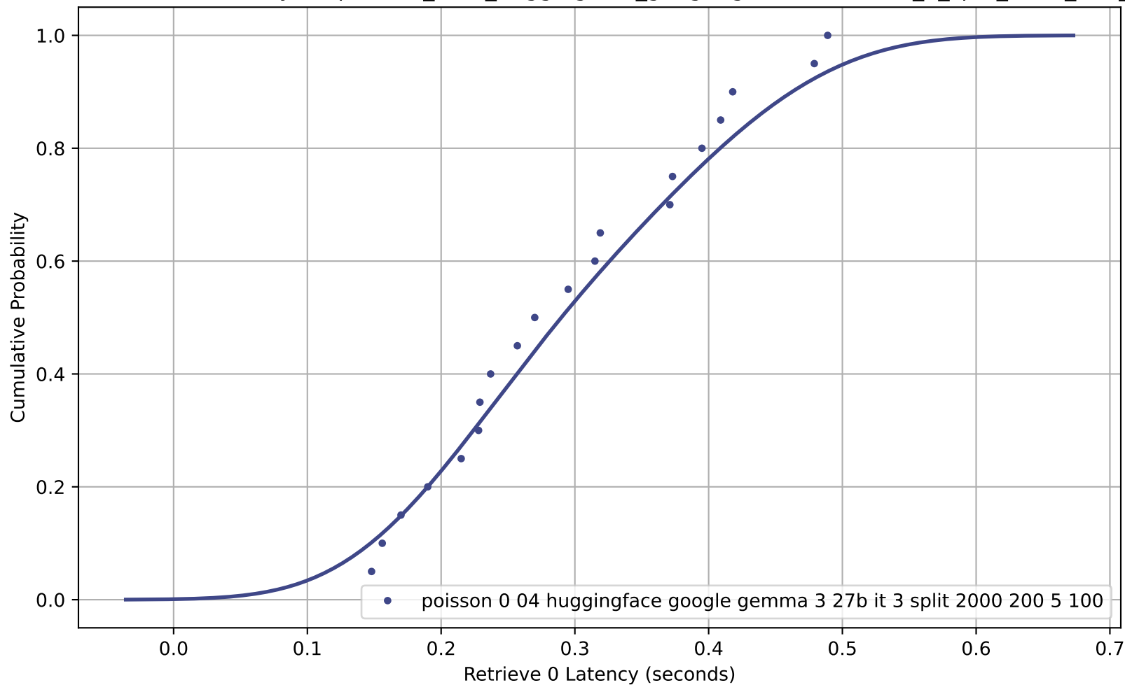
CDF of Retrieve 0 Latency for poisson_0-04_huggingface_google-gemma-3-27b-it_3_split_2000_200_5_100
