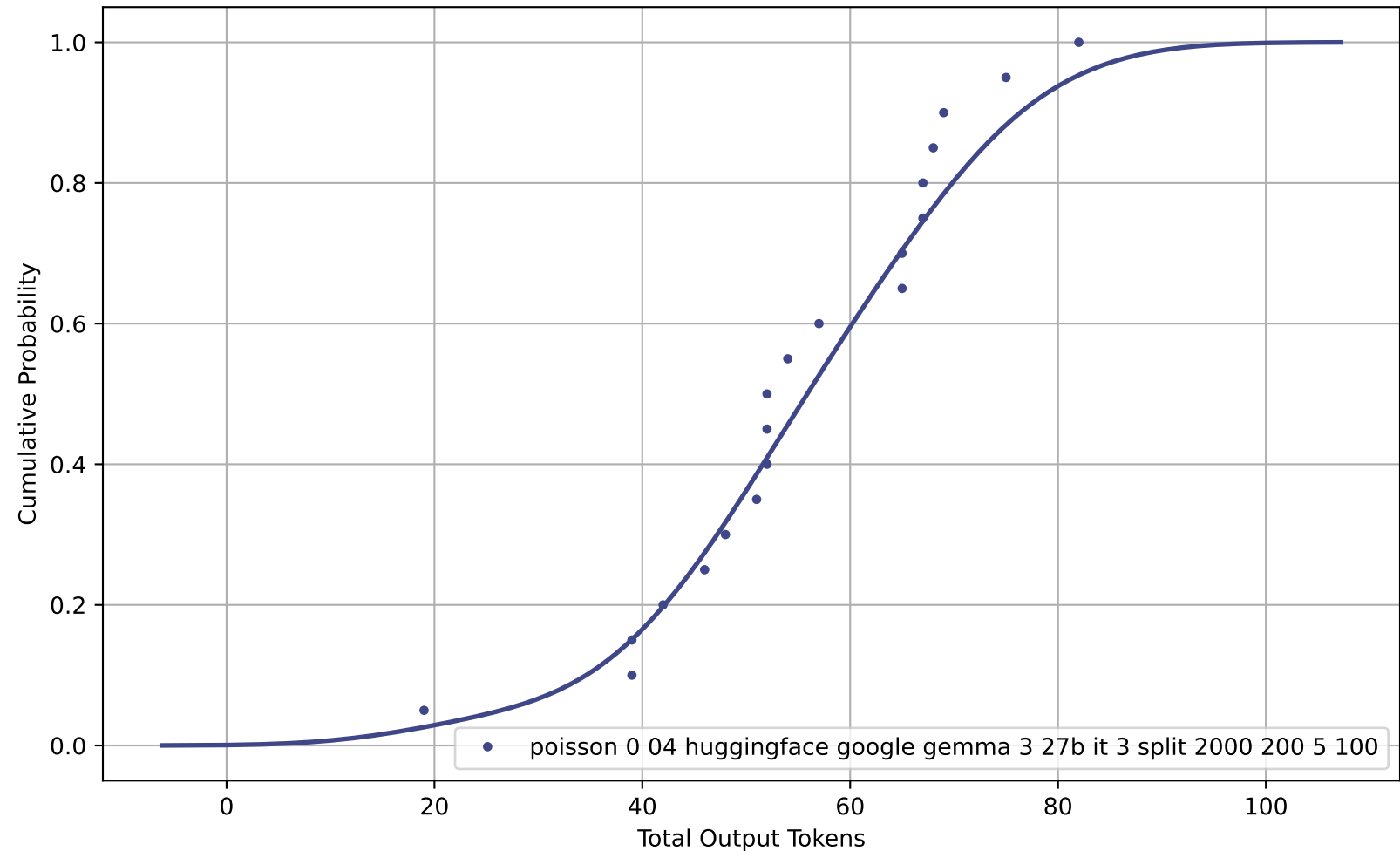
CDF of Total Output Tokens for poisson_0-04_huggingface_google-gemma-3-27b-it_3_split_2000_200_5_100
