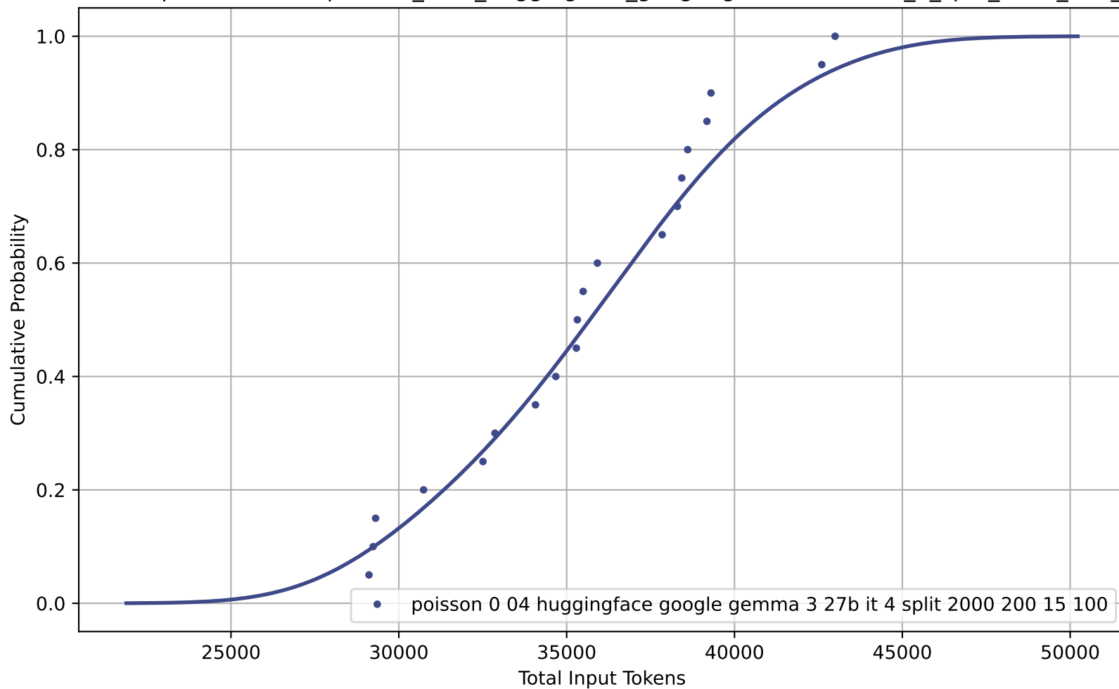
CDF of Total Input Tokens for poisson_0-04_huggingface_google-gemma-3-27b-it_4_split_2000_200_15_100
