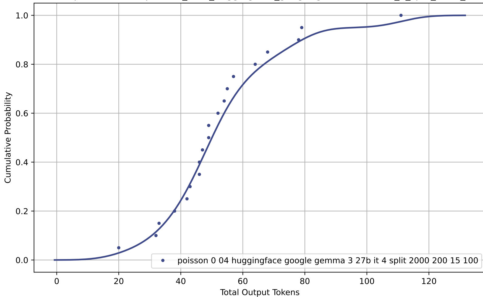
CDF of Total Output Tokens for poisson_0-04_huggingface_google-gemma-3-27b-it_4_split_2000_200_15_100
