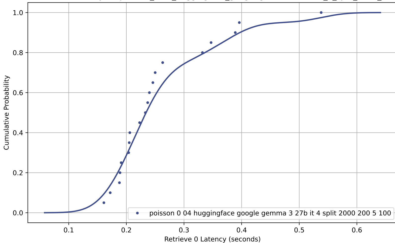
CDF of Retrieve 0 Latency for poisson_0-04_huggingface_google-gemma-3-27b-it_4_split_2000_200_5_100
