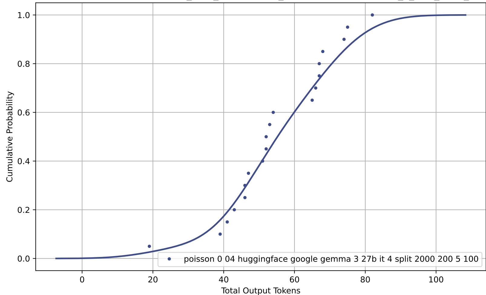
CDF of Total Output Tokens for poisson_0-04_huggingface_google-gemma-3-27b-it_4_split_2000_200_5_100
