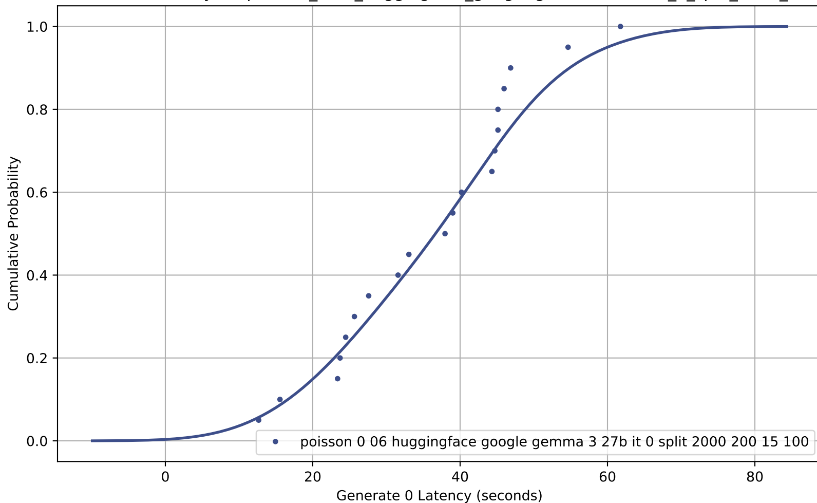
CDF of Generate 0 Latency for poisson_0-06_huggingface_google-gemma-3-27b-it_0_split_2000_200_15_100
