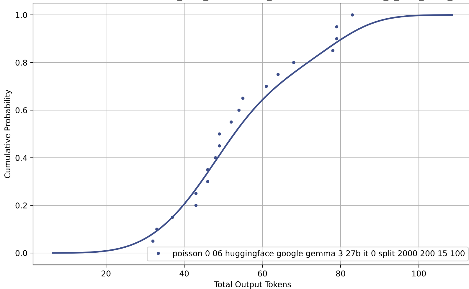
CDF of Total Output Tokens for poisson_0-06_huggingface_google-gemma-3-27b-it_0_split_2000_200_15_100
