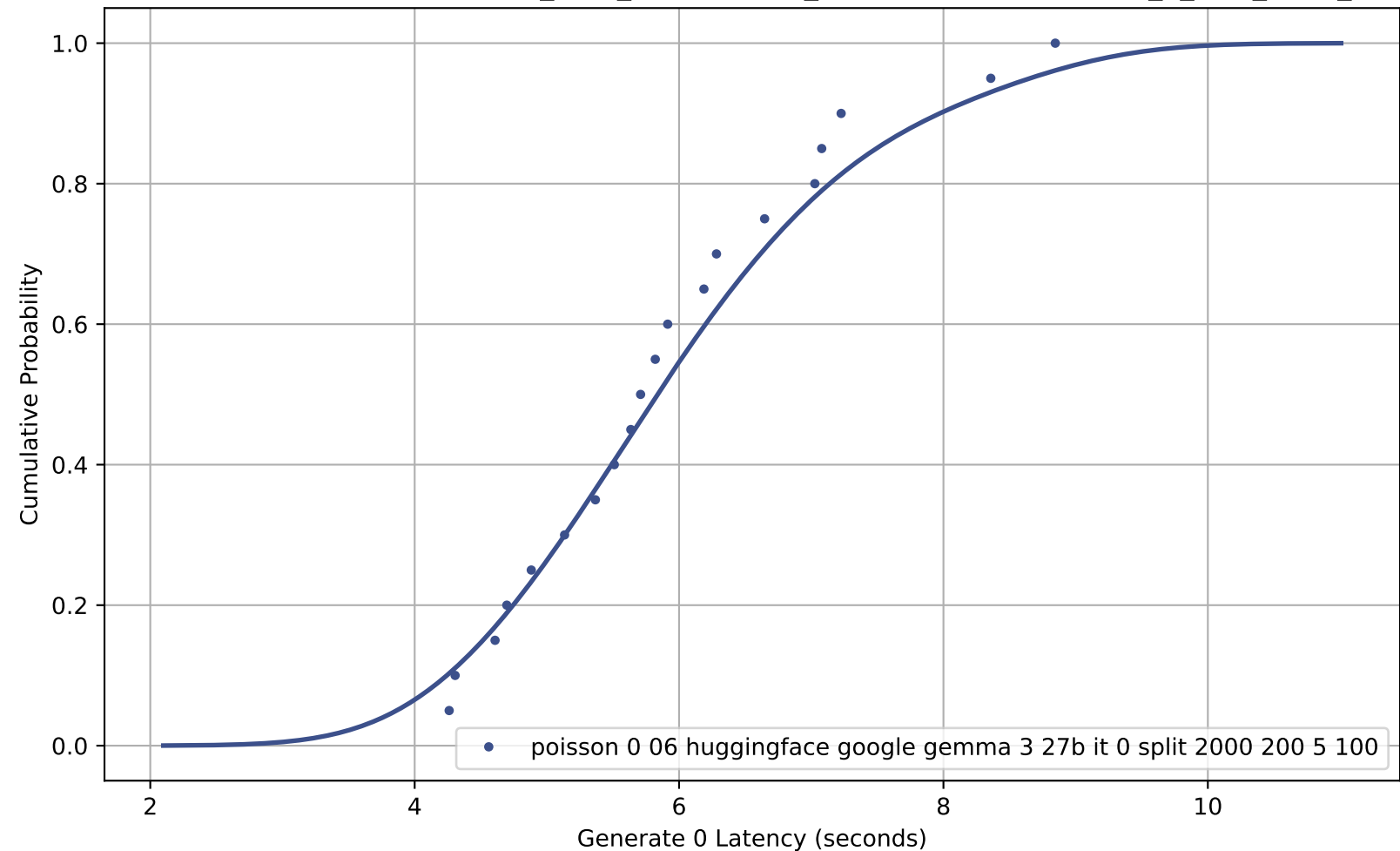
CDF of Generate 0 Latency for poisson_0-06_huggingface_google-gemma-3-27b-it_0_split_2000_200_5_100
