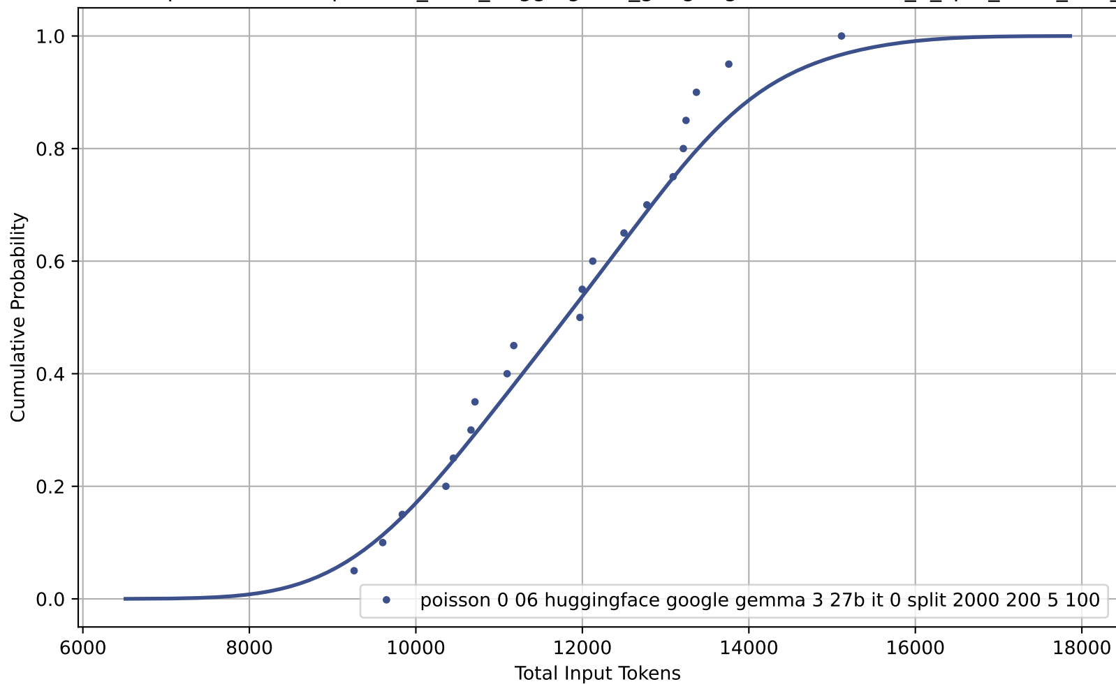
CDF of Total Input Tokens for poisson_0-06_huggingface_google-gemma-3-27b-it_0_split_2000_200_5_100
