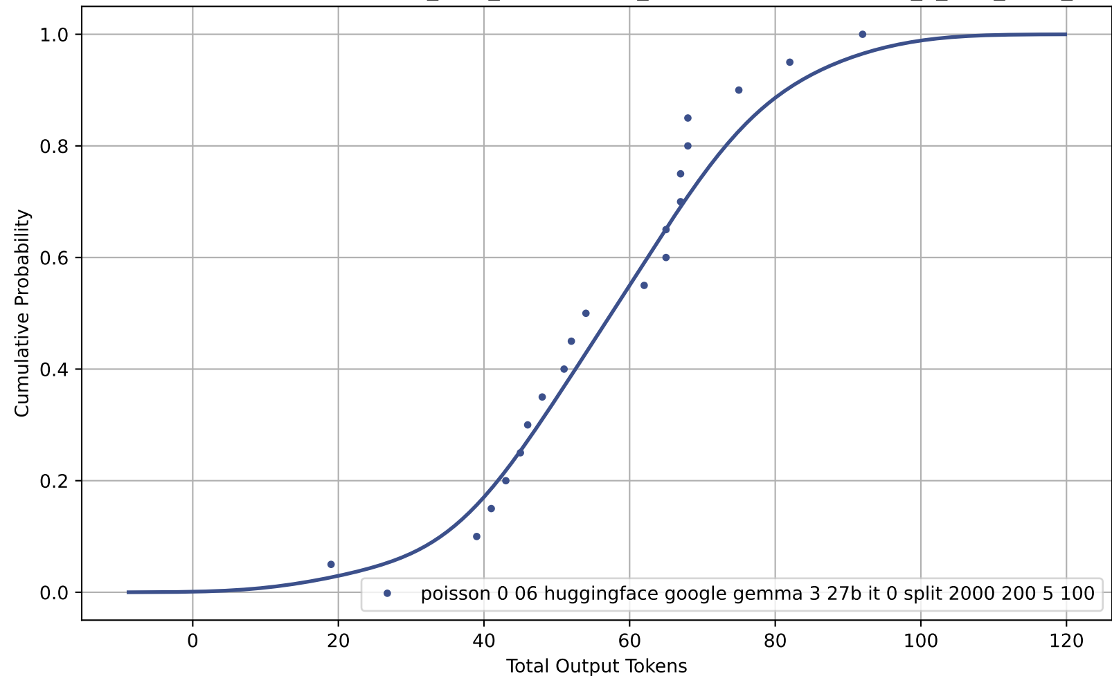
CDF of Total Output Tokens for poisson_0-06_huggingface_google-gemma-3-27b-it_0_split_2000_200_5_100
