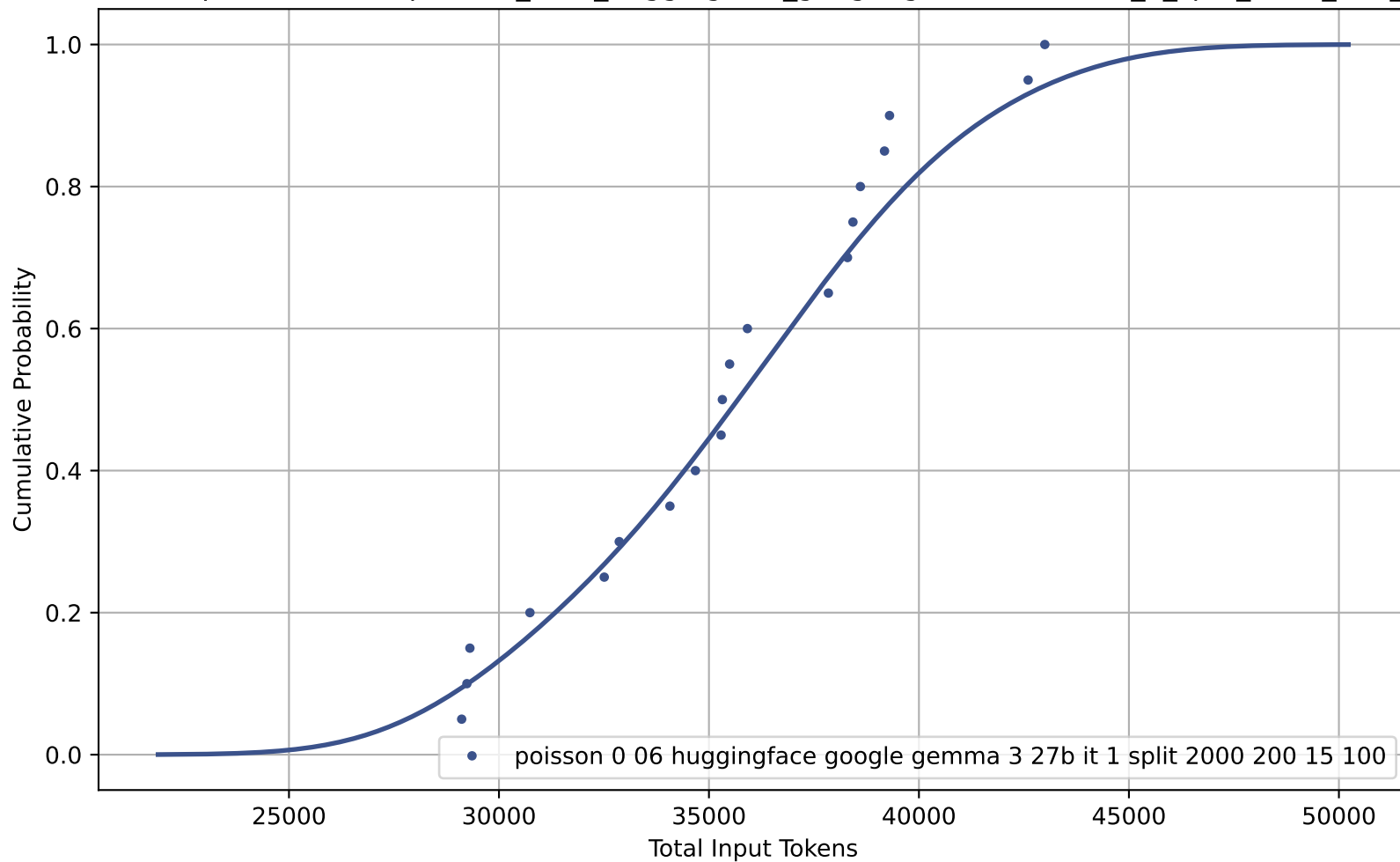
CDF of Total Input Tokens for poisson_0-06_huggingface_google-gemma-3-27b-it_1_split_2000_200_15_100
