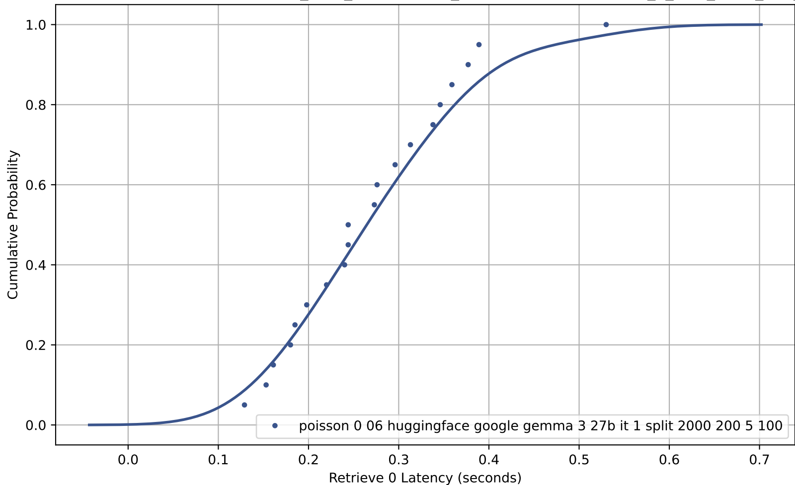
CDF of Retrieve 0 Latency for poisson_0-06_huggingface_google-gemma-3-27b-it_1_split_2000_200_5_100
