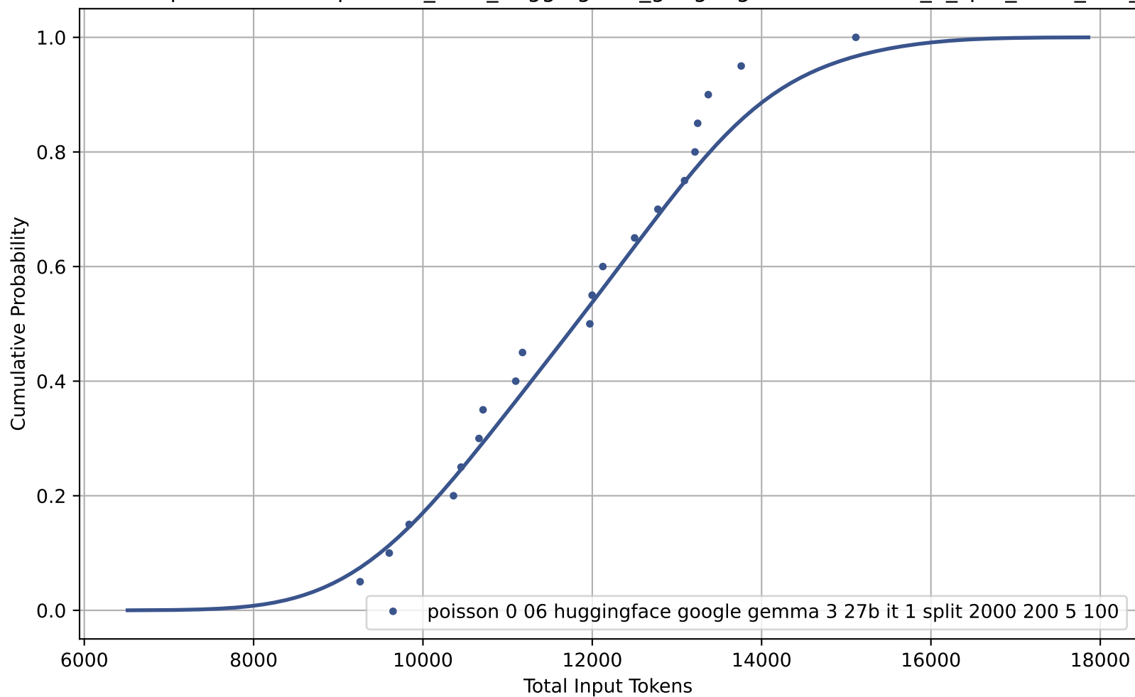
CDF of Total Input Tokens for poisson_0-06_huggingface_google-gemma-3-27b-it_1_split_2000_200_5_100
