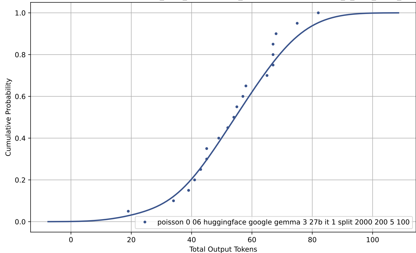
CDF of Total Output Tokens for poisson_0-06_huggingface_google-gemma-3-27b-it_1_split_2000_200_5_100
