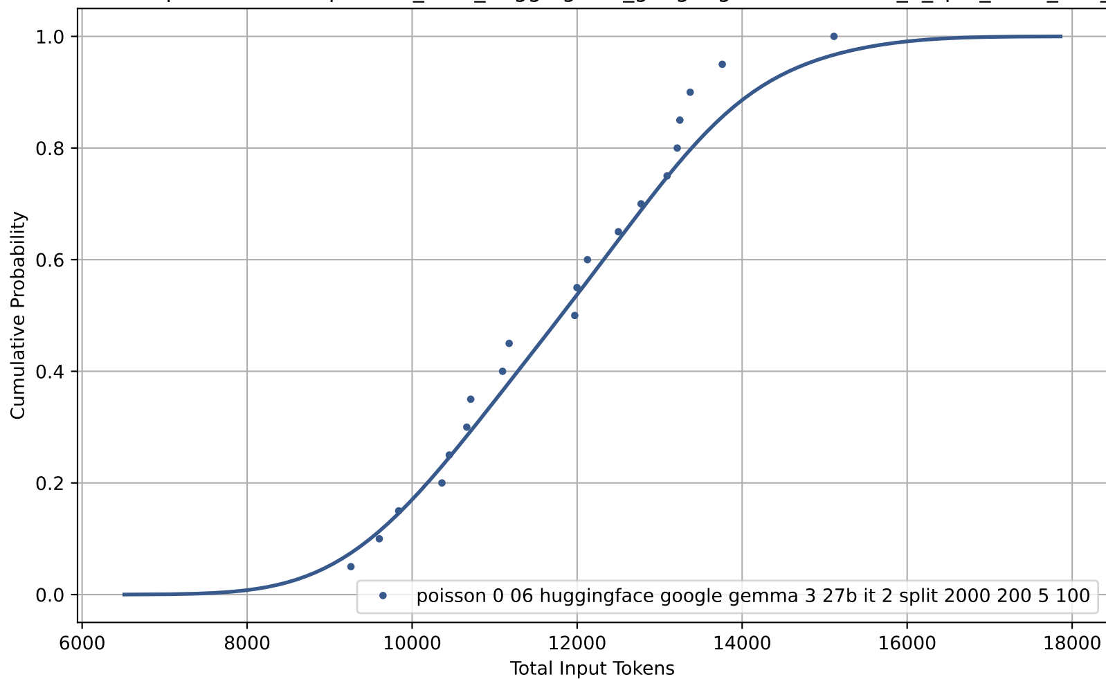
CDF of Total Input Tokens for poisson_0-06_huggingface_google-gemma-3-27b-it_2_split_2000_200_5_100
