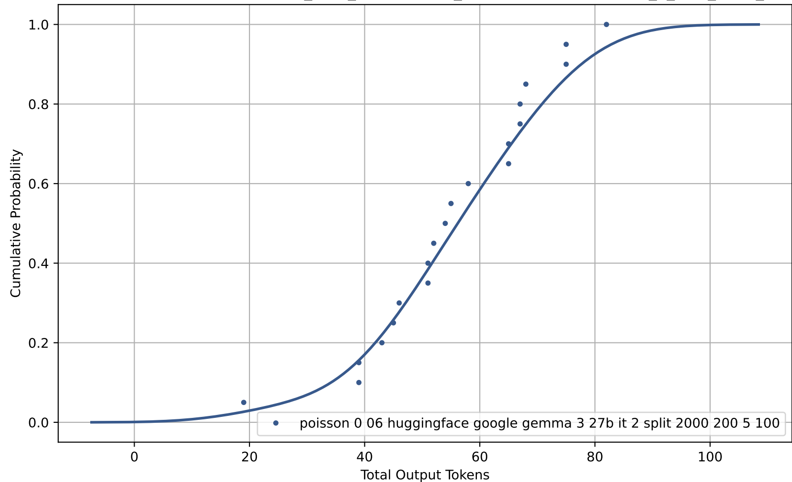
CDF of Total Output Tokens for poisson_0-06_huggingface_google-gemma-3-27b-it_2_split_2000_200_5_100
