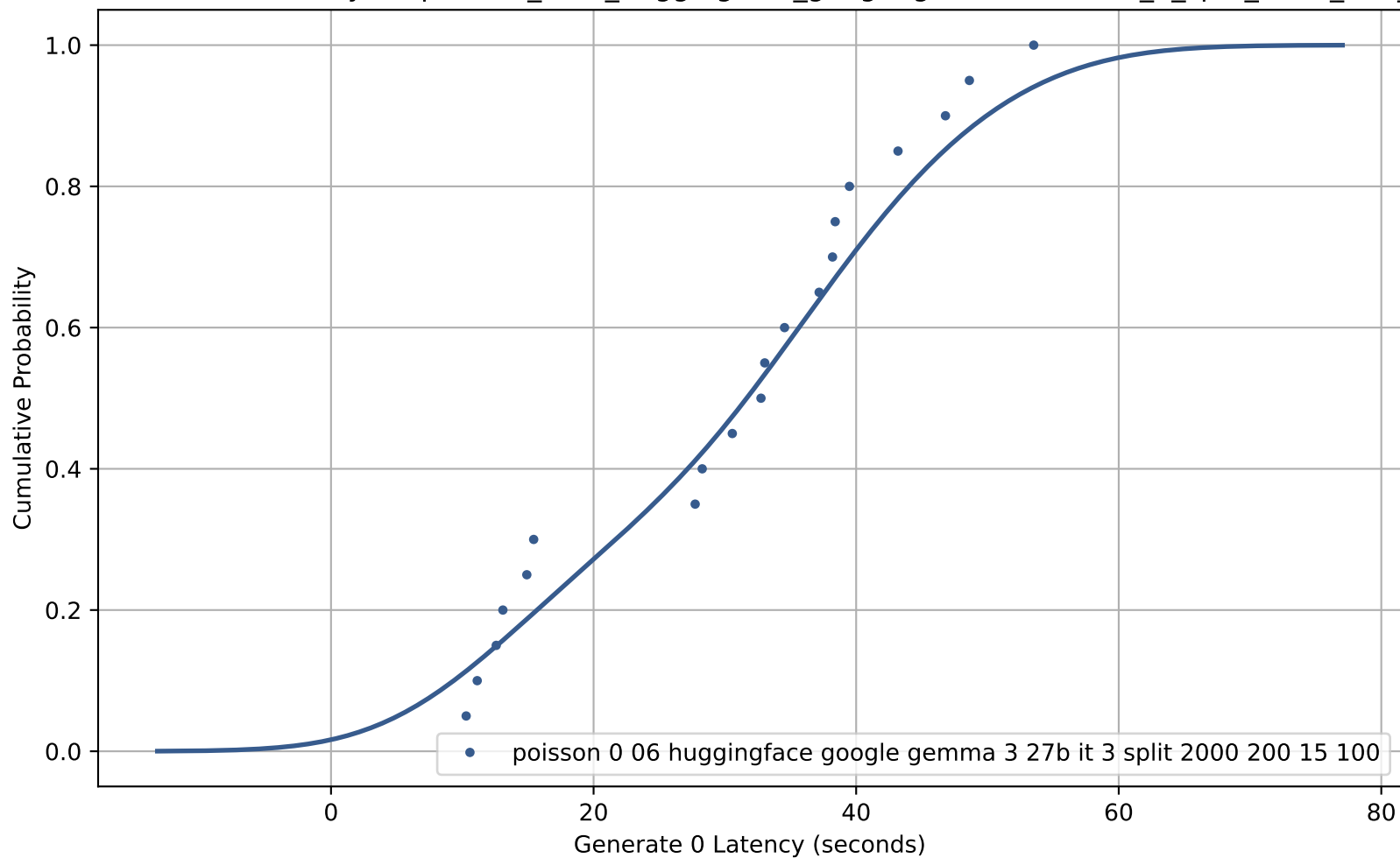
CDF of Generate 0 Latency for poisson_0-06_huggingface_google-gemma-3-27b-it_3_split_2000_200_15_100
