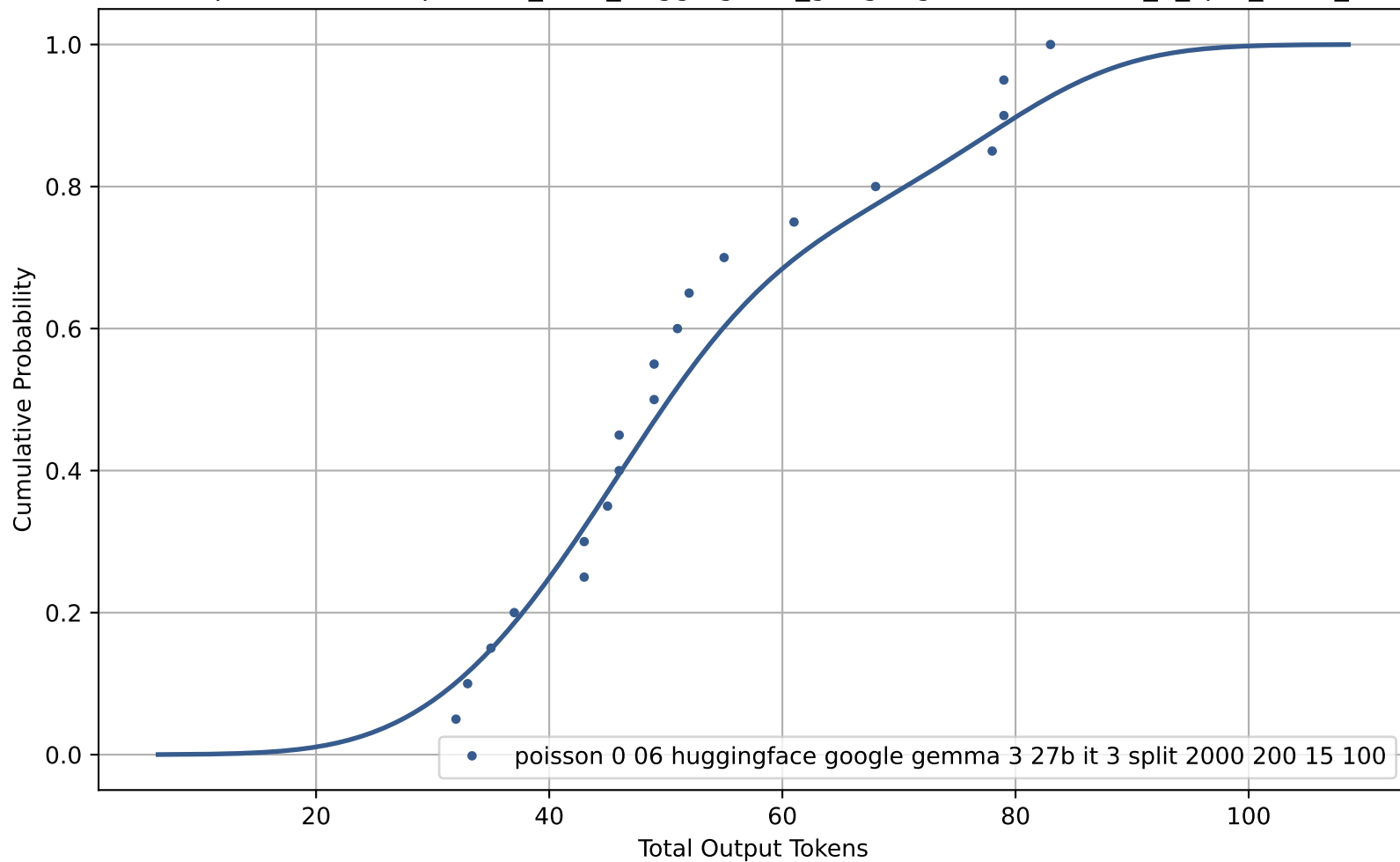
CDF of Total Output Tokens for poisson_0-06_huggingface_google-gemma-3-27b-it_3_split_2000_200_15_100
