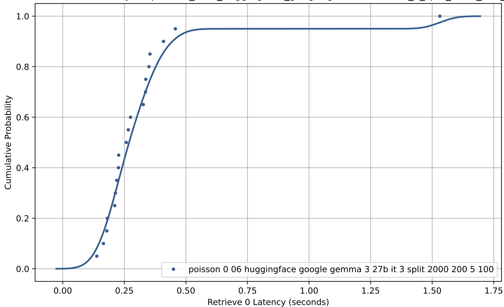
CDF of Retrieve 0 Latency for poisson_0-06_huggingface_google-gemma-3-27b-it_3_split_2000_200_5_100
