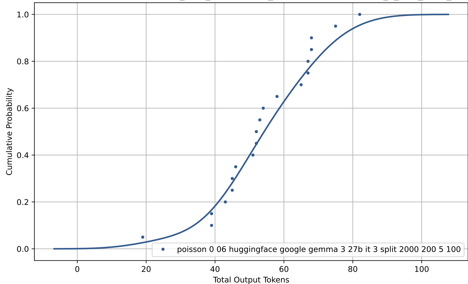
CDF of Total Output Tokens for poisson_0-06_huggingface_google-gemma-3-27b-it_3_split_2000_200_5_100
