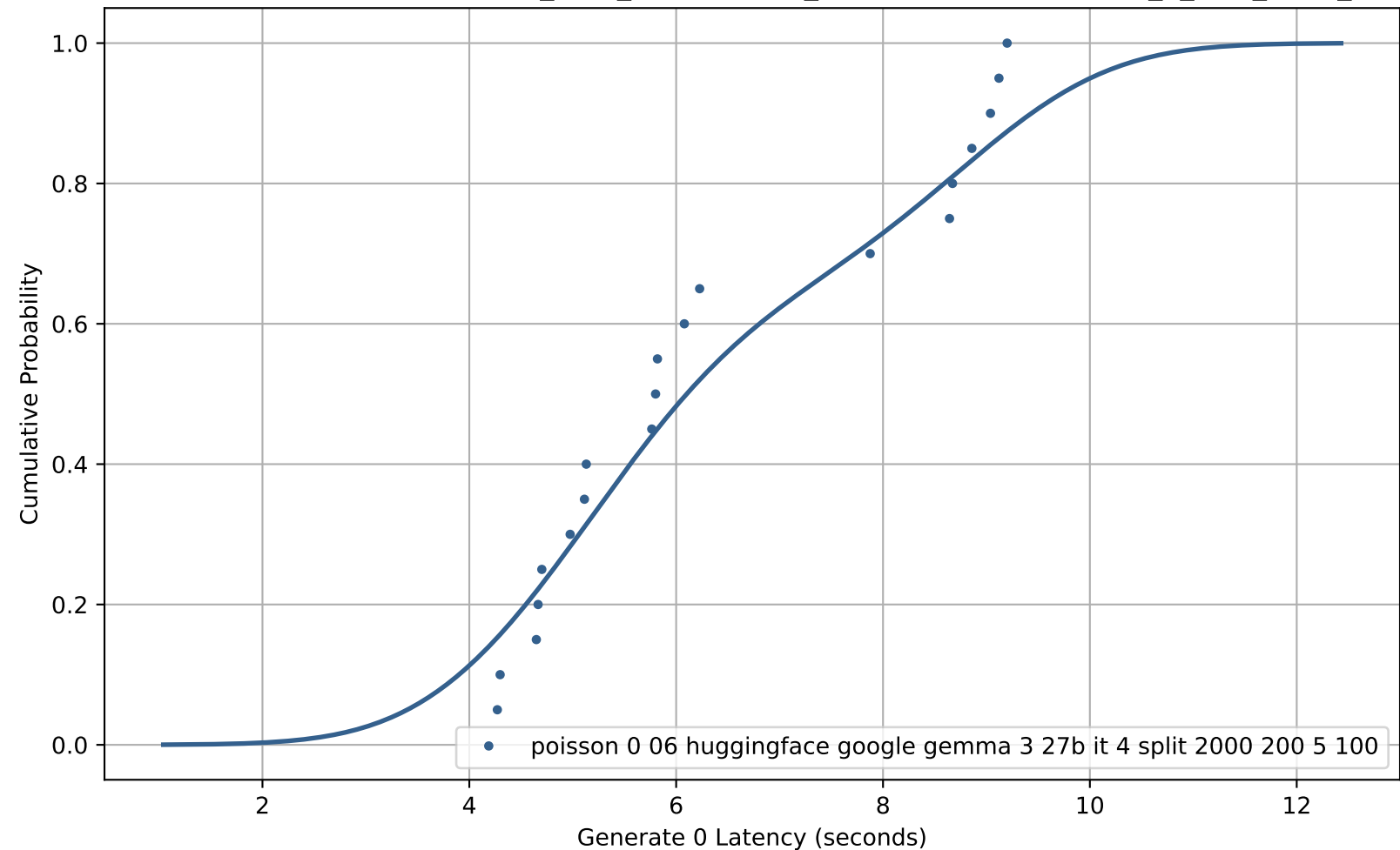
CDF of Generate 0 Latency for poisson_0-06_huggingface_google-gemma-3-27b-it_4_split_2000_200_5_100
