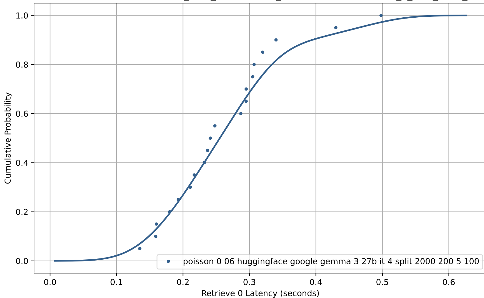
CDF of Retrieve 0 Latency for poisson_0-06_huggingface_google-gemma-3-27b-it_4_split_2000_200_5_100
