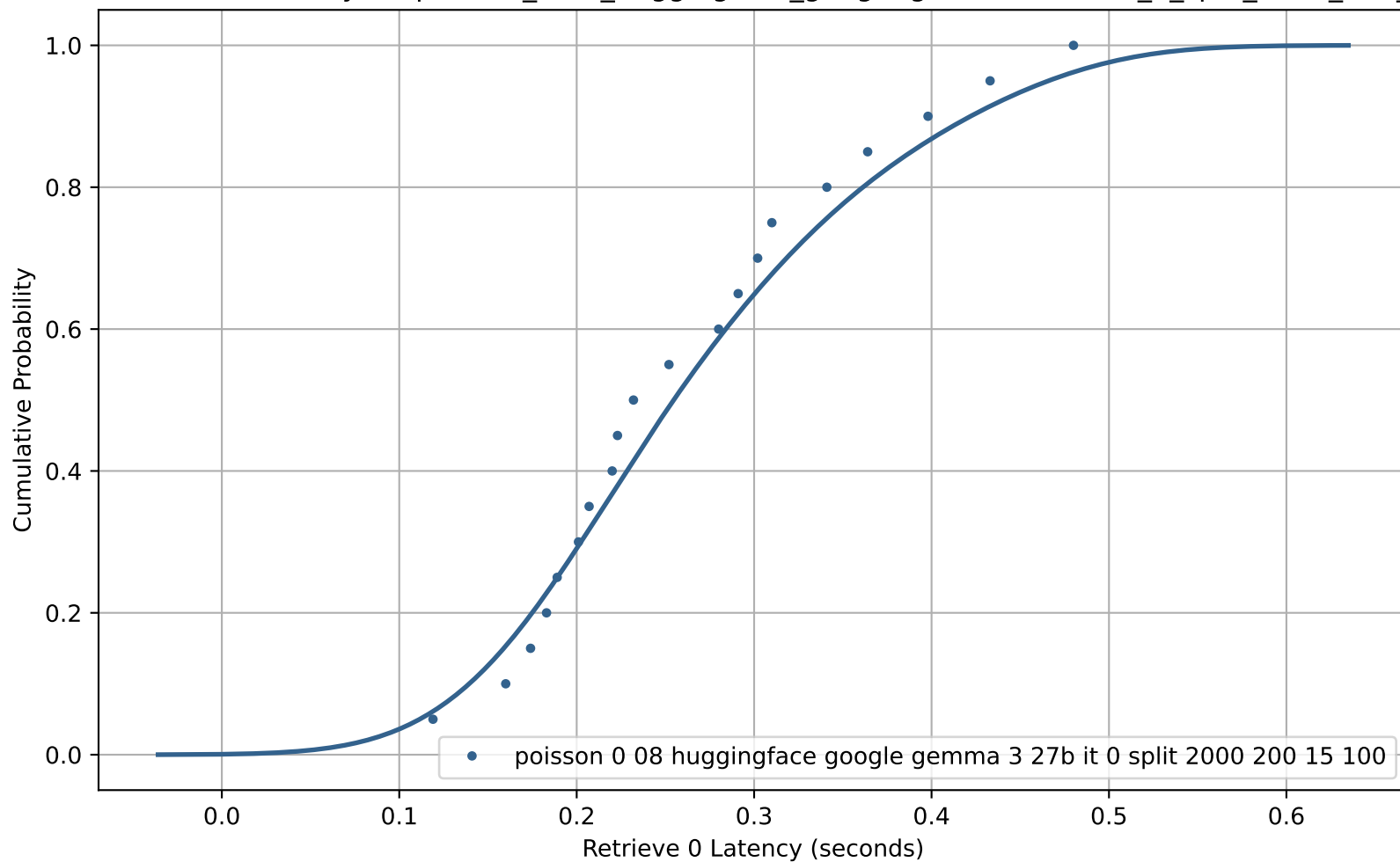
CDF of Retrieve 0 Latency for poisson_0-08_huggingface_google-gemma-3-27b-it_0_split_2000_200_15_100
