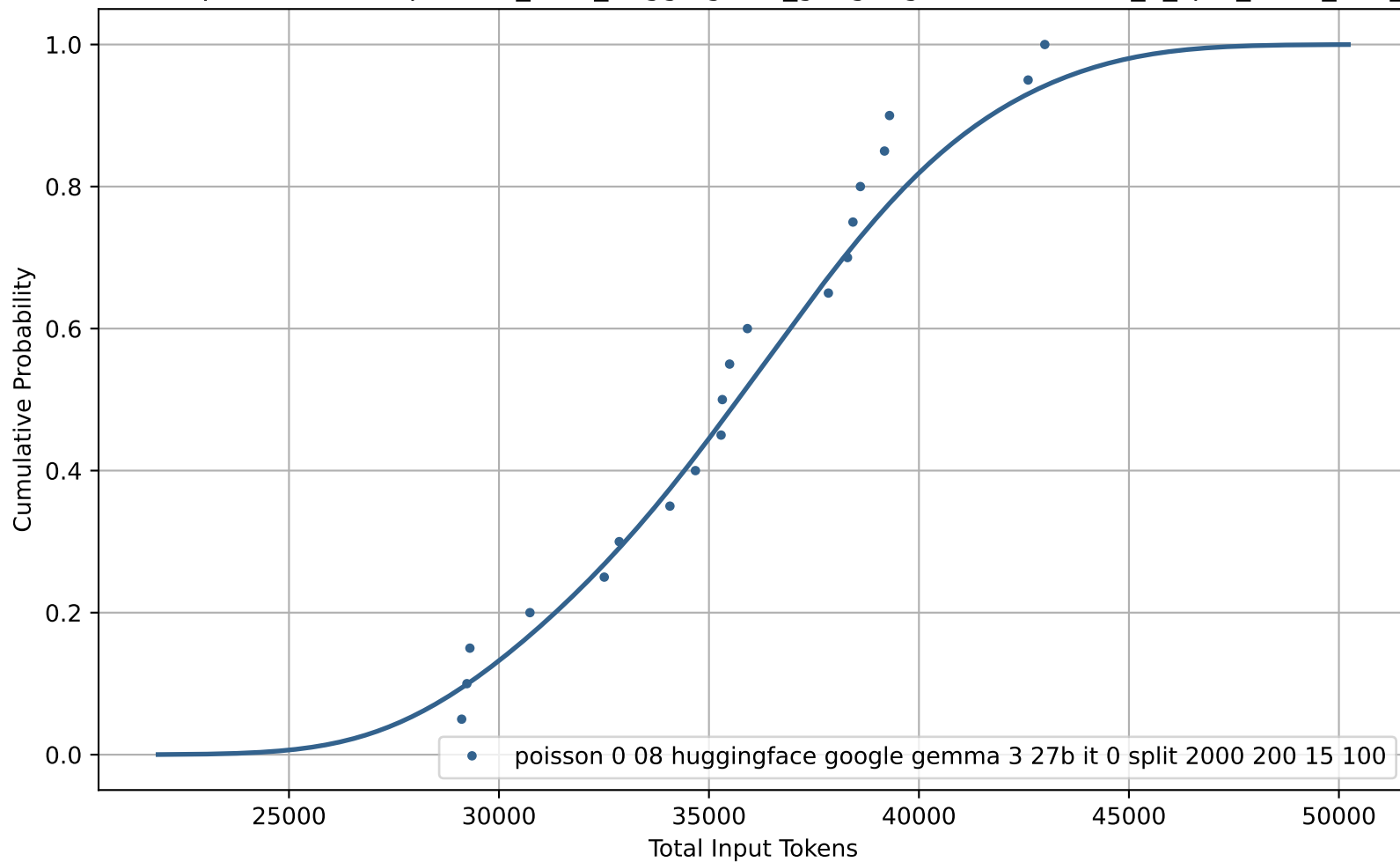
CDF of Total Input Tokens for poisson_0-08_huggingface_google-gemma-3-27b-it_0_split_2000_200_15_100
