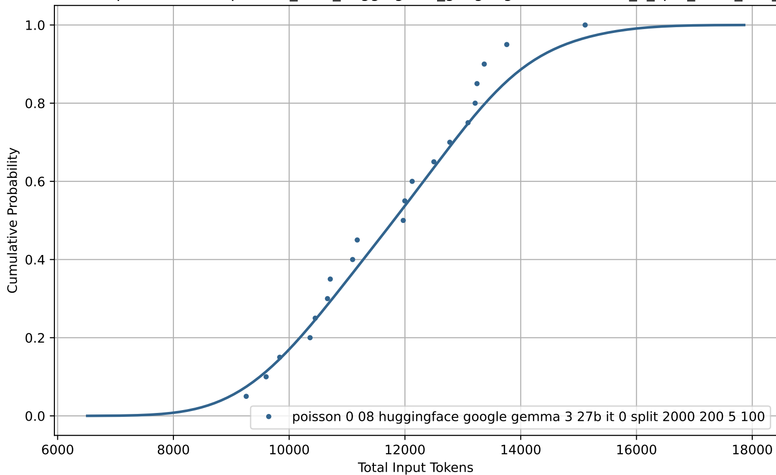
CDF of Total Input Tokens for poisson_0-08_huggingface_google-gemma-3-27b-it_0_split_2000_200_5_100
