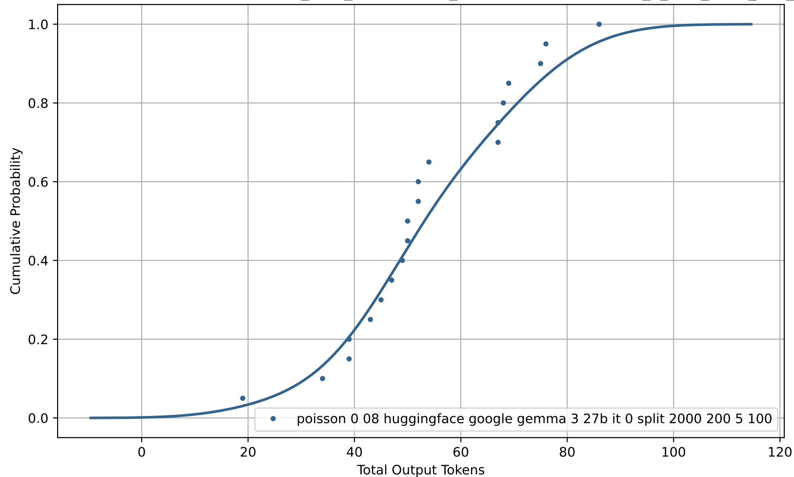
CDF of Total Output Tokens for poisson_0-08_huggingface_google-gemma-3-27b-it_0_split_2000_200_5_100
