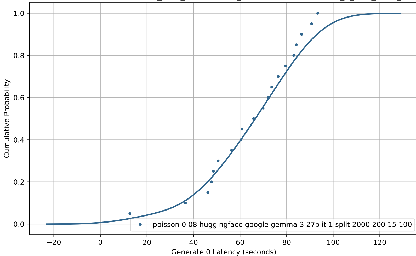
CDF of Generate 0 Latency for poisson_0-08_huggingface_google-gemma-3-27b-it_1_split_2000_200_15_100
