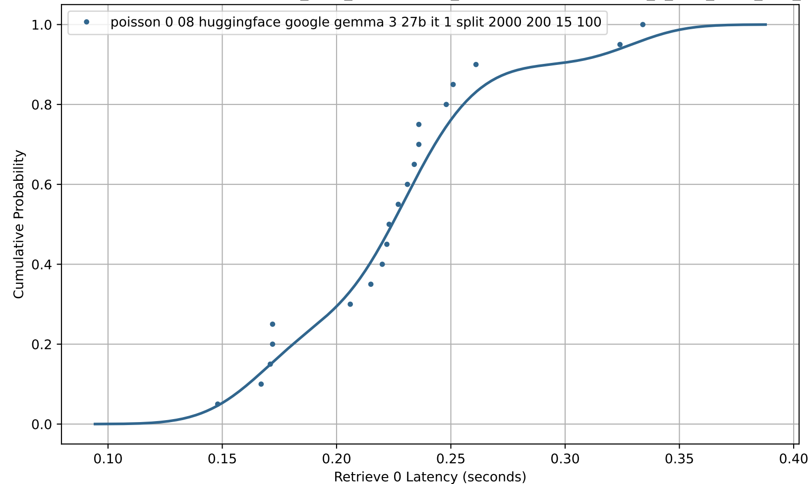
CDF of Retrieve 0 Latency for poisson_0-08_huggingface_google-gemma-3-27b-it_1_split_2000_200_15_100
