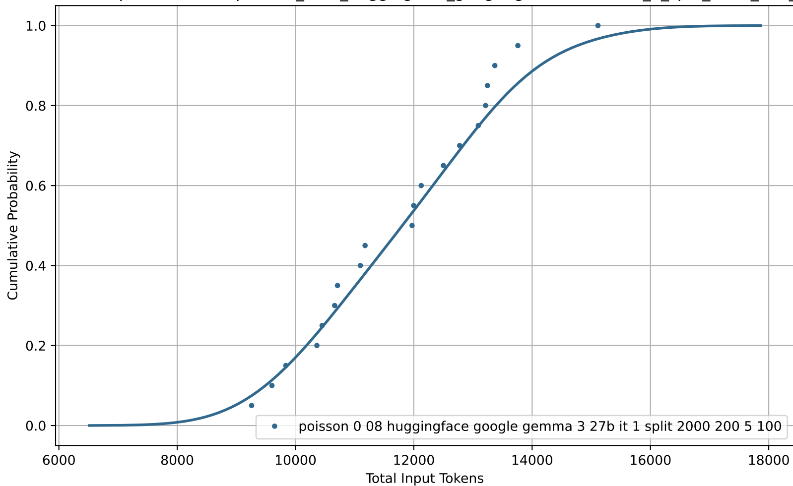
CDF of Total Input Tokens for poisson_0-08_huggingface_google-gemma-3-27b-it_1_split_2000_200_5_100
