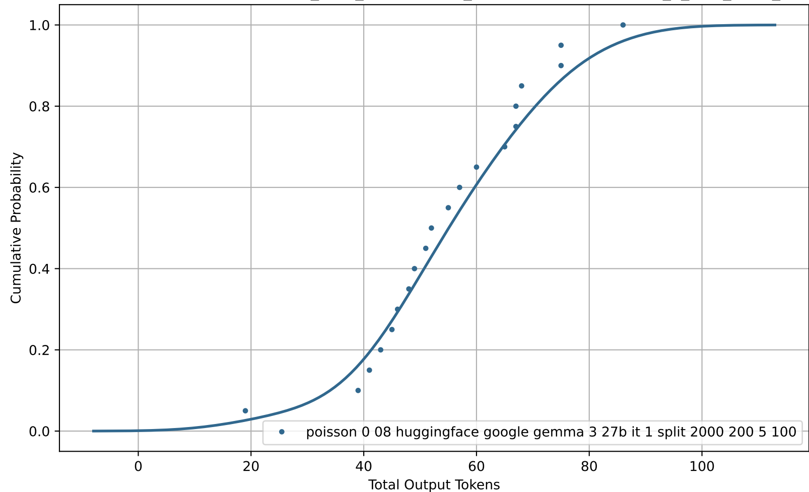
CDF of Total Output Tokens for poisson_0-08_huggingface_google-gemma-3-27b-it_1_split_2000_200_5_100
