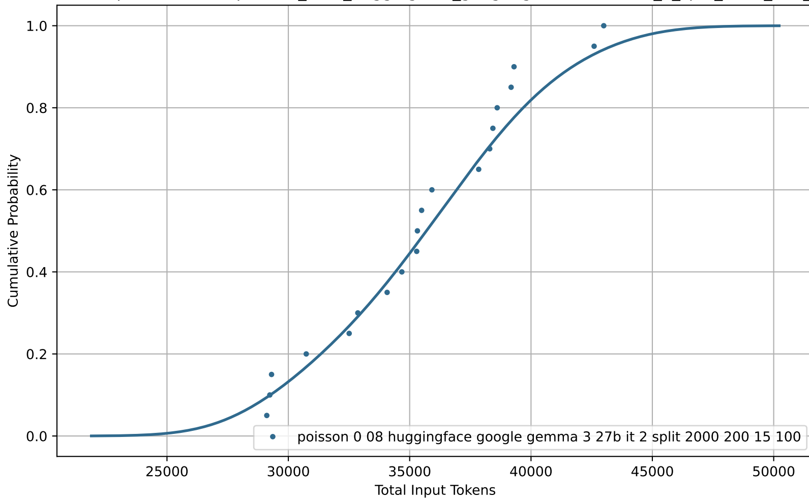
CDF of Total Input Tokens for poisson_0-08_huggingface_google-gemma-3-27b-it_2_split_2000_200_15_100
