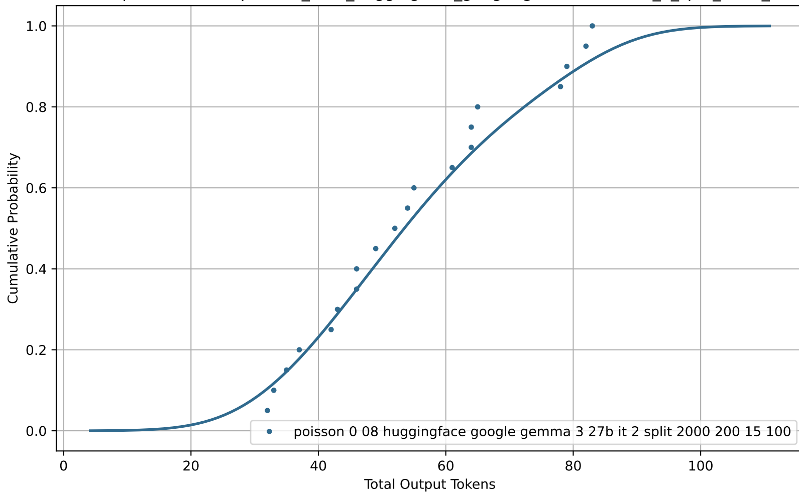
CDF of Total Output Tokens for poisson_0-08_huggingface_google-gemma-3-27b-it_2_split_2000_200_15_100
