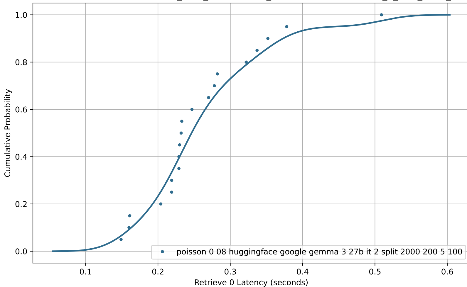
CDF of Retrieve 0 Latency for poisson_0-08_huggingface_google-gemma-3-27b-it_2_split_2000_200_5_100
