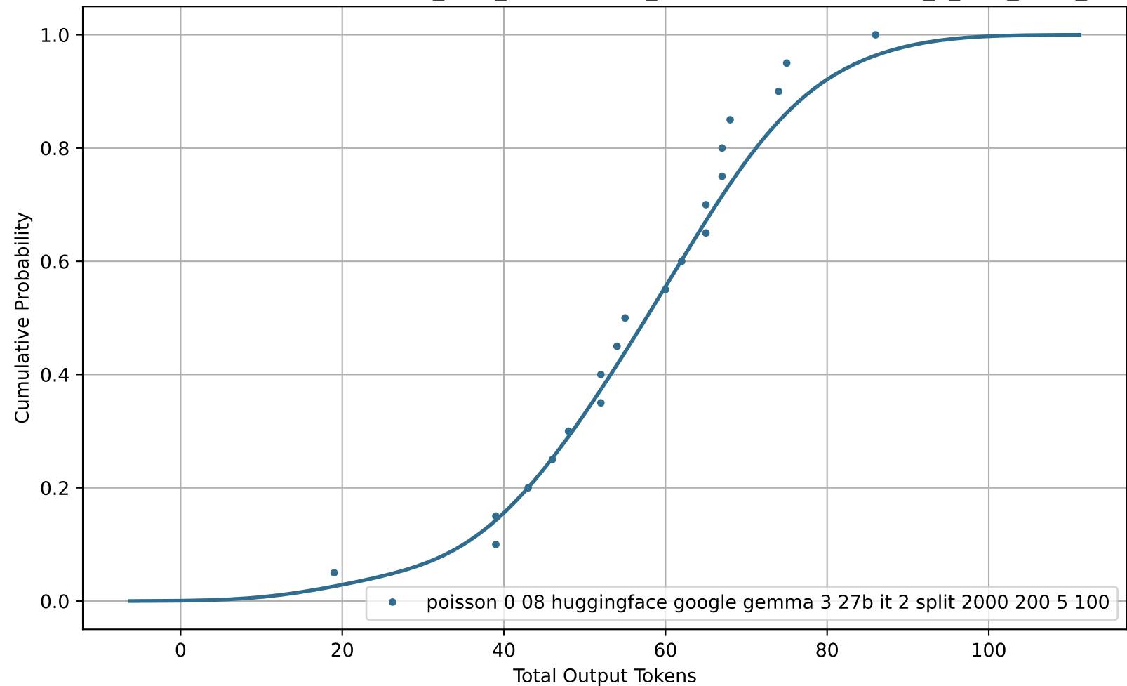
CDF of Total Output Tokens for poisson_0-08_huggingface_google-gemma-3-27b-it_2_split_2000_200_5_100
