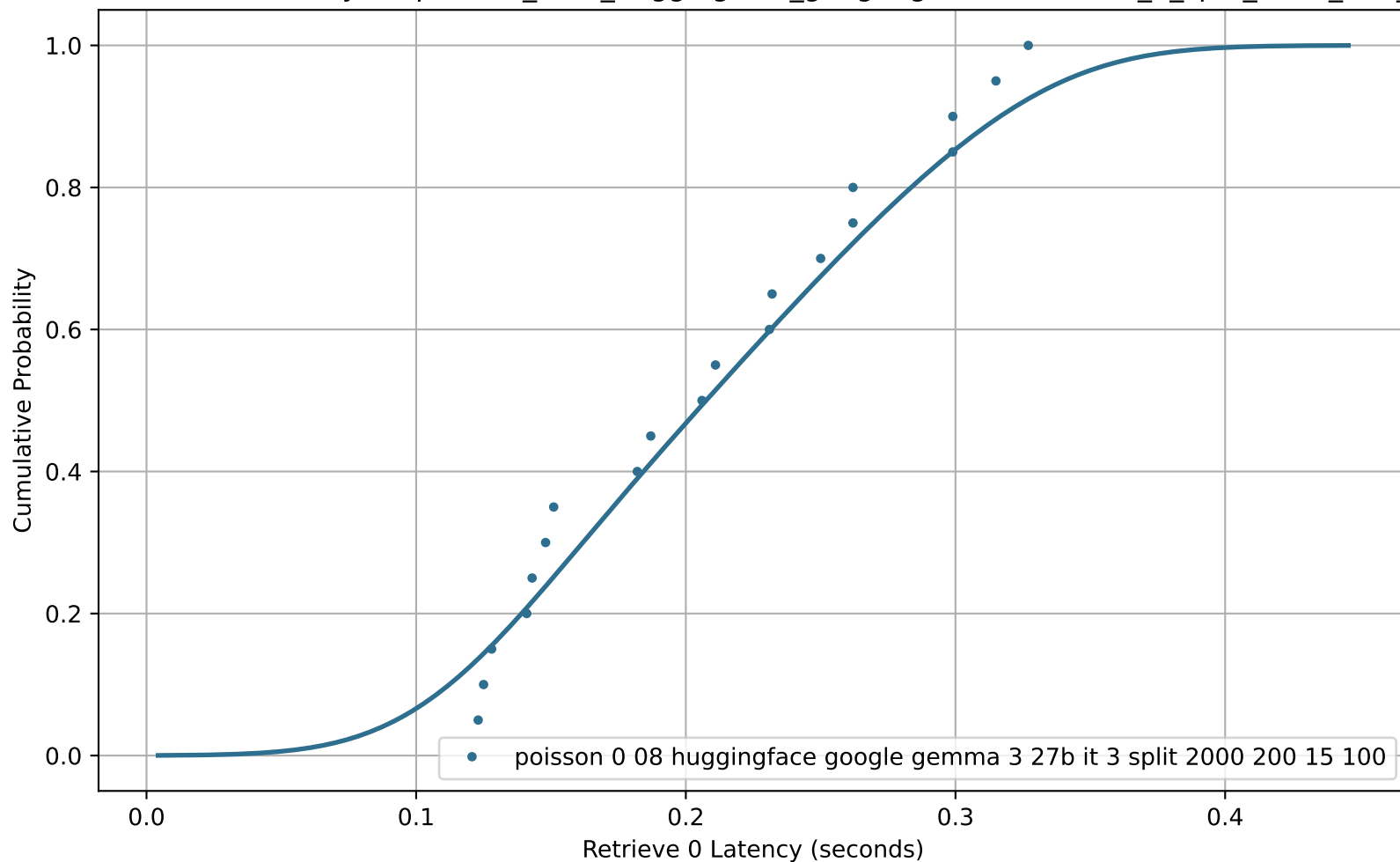
CDF of Retrieve 0 Latency for poisson_0-08_huggingface_google-gemma-3-27b-it_3_split_2000_200_15_100
