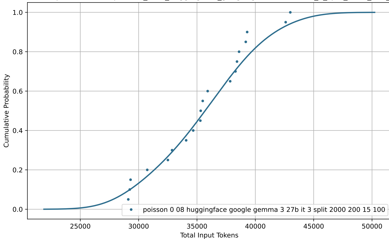
CDF of Total Input Tokens for poisson_0-08_huggingface_google-gemma-3-27b-it_3_split_2000_200_15_100
