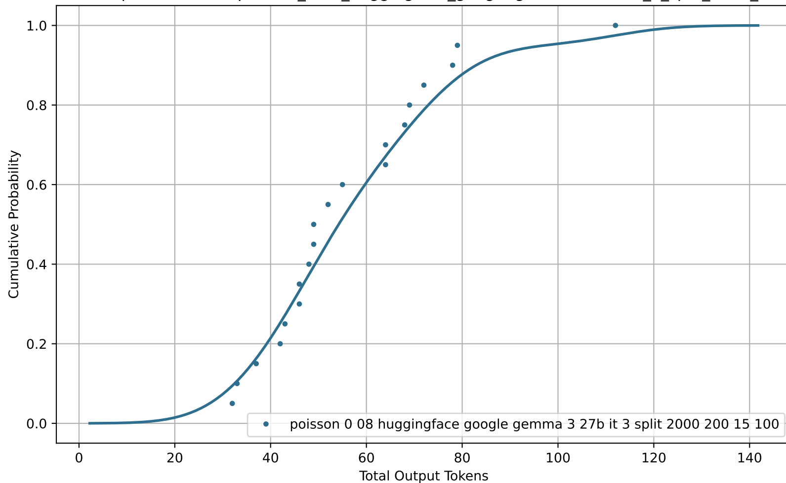
CDF of Total Output Tokens for poisson_0-08_huggingface_google-gemma-3-27b-it_3_split_2000_200_15_100
