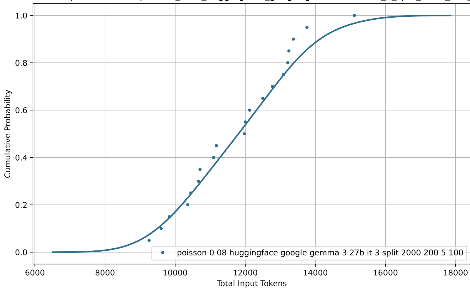
CDF of Total Input Tokens for poisson_0-08_huggingface_google-gemma-3-27b-it_3_split_2000_200_5_100
