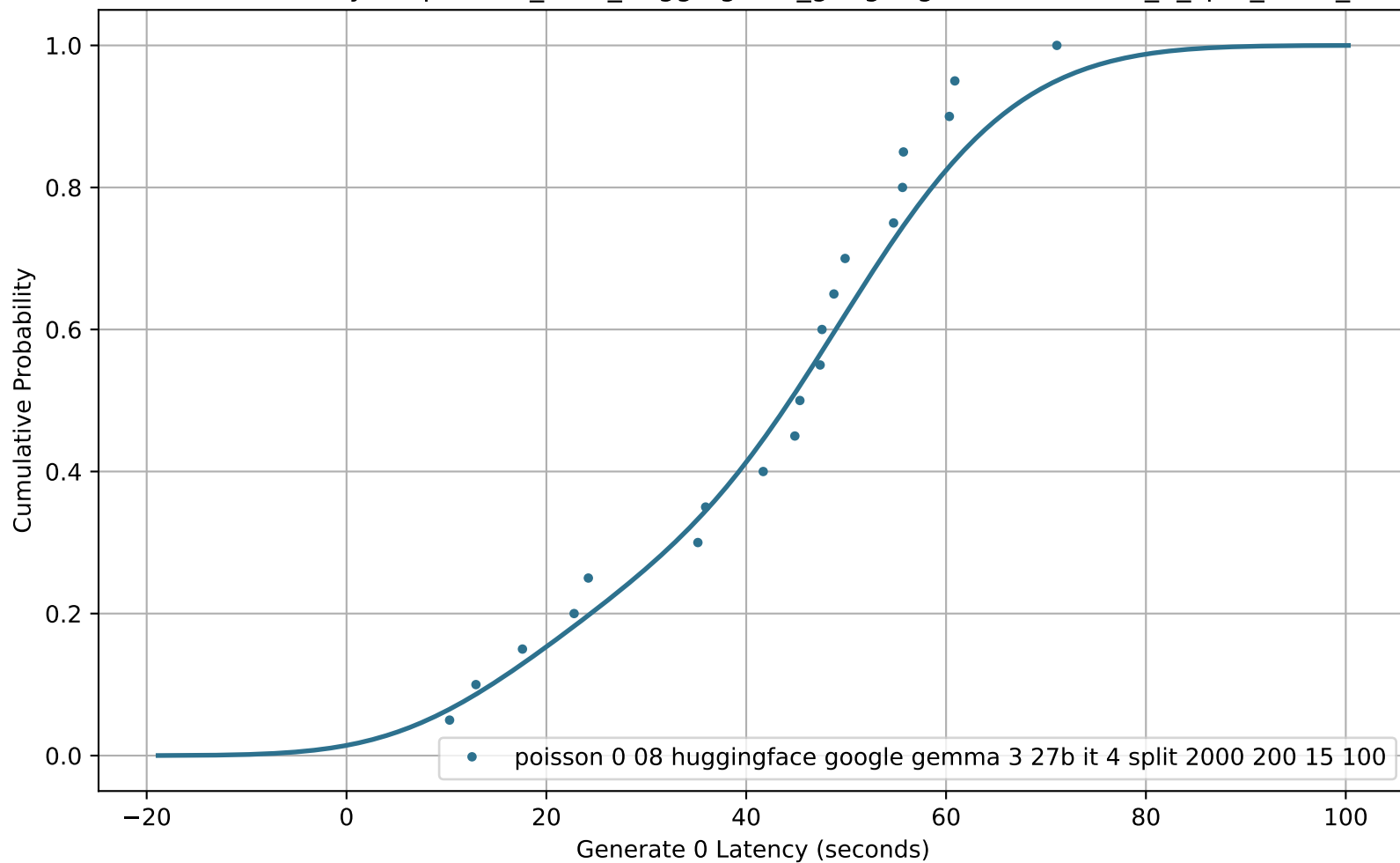
CDF of Generate 0 Latency for poisson_0-08_huggingface_google-gemma-3-27b-it_4_split_2000_200_15_100
